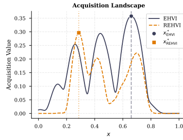
(b) Acquisition Functions
