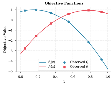
(a) Underlying Objective Functions
